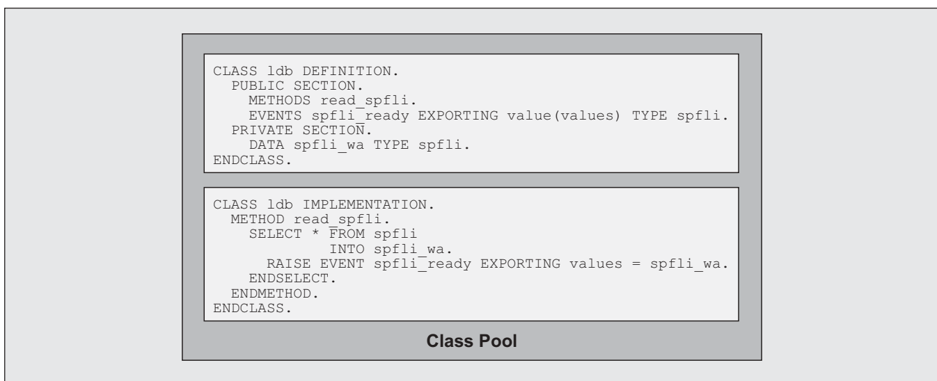
Figure 18 Simplifying a Logical Database with ABAP Objects
