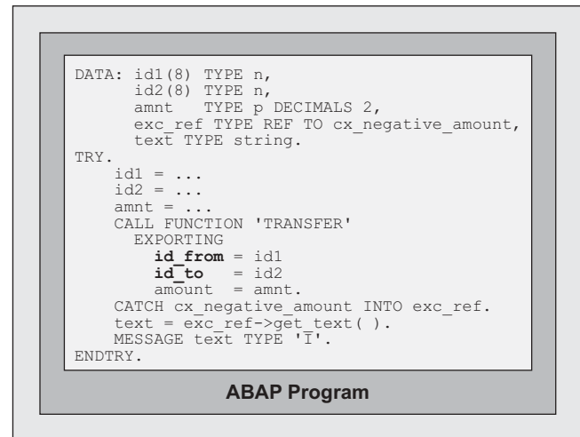
Figure 4 Implicit Instantiation of a Function Pool
